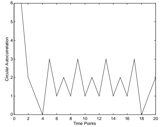
Figure 1. Circular Autocorrelation Function when the length is a multiple of the period
