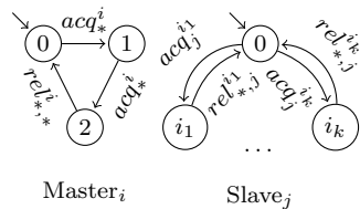
Fig. 8. Master Slave example
