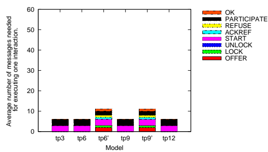
Fig. 15. Transmission protocol: Number of messages per interaction, optimized version.
